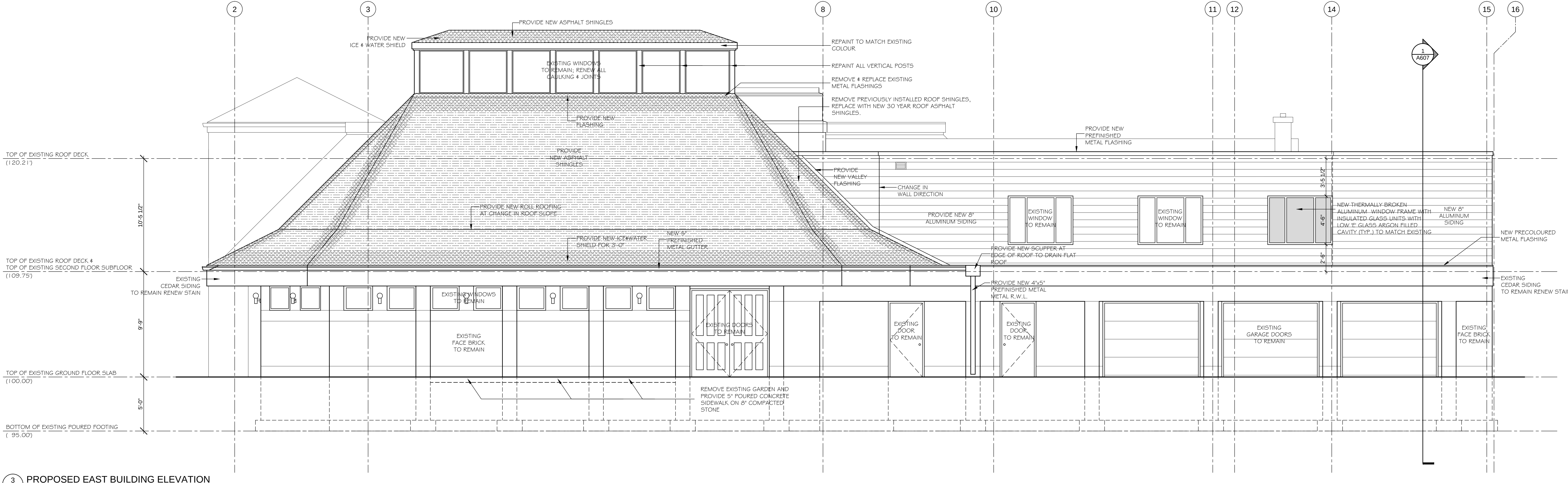
3 PROPOSED EAST BUILDING ELEVATION A401 3/4" = 1'-0"
