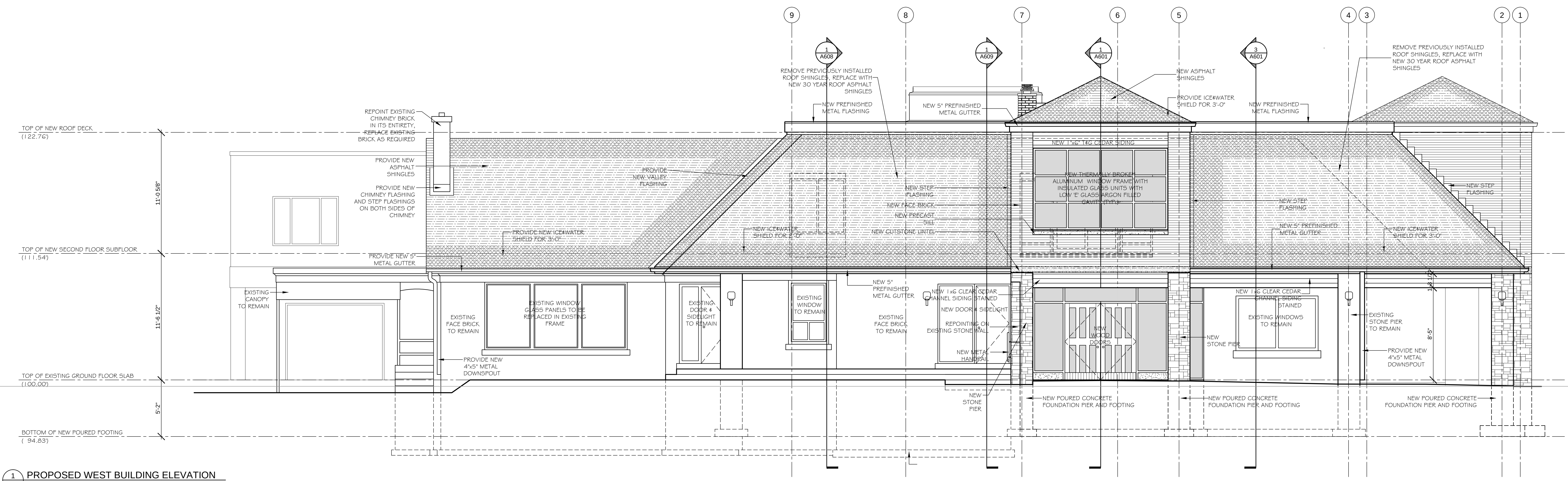
1 PROPOSED WEST BUILDING ELEVATION A401 3/4" = 1'-0"
