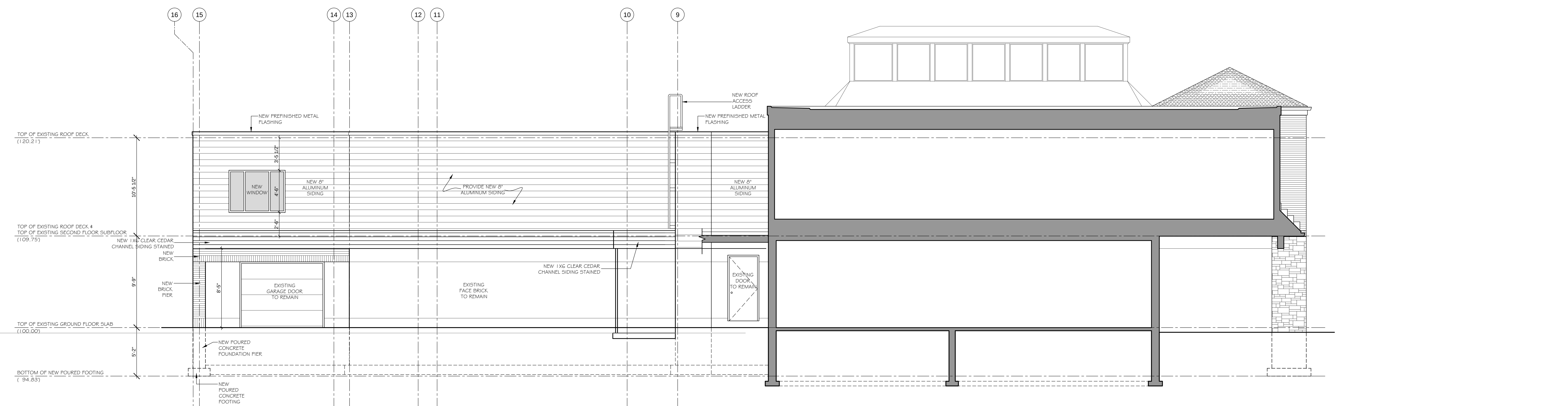
3 PROPOSED WEST BUILDING ELEVATION A402 3/4" = 1'-0"
