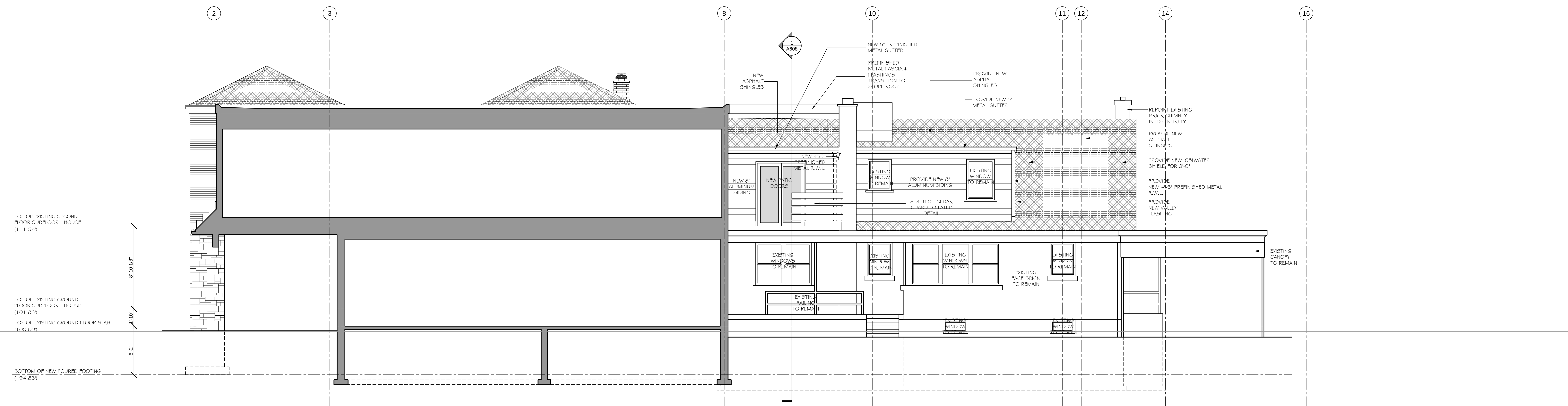
2 PROPOSED EAST BUILDING ELEVATION A402 3/4" = 1'-0"
