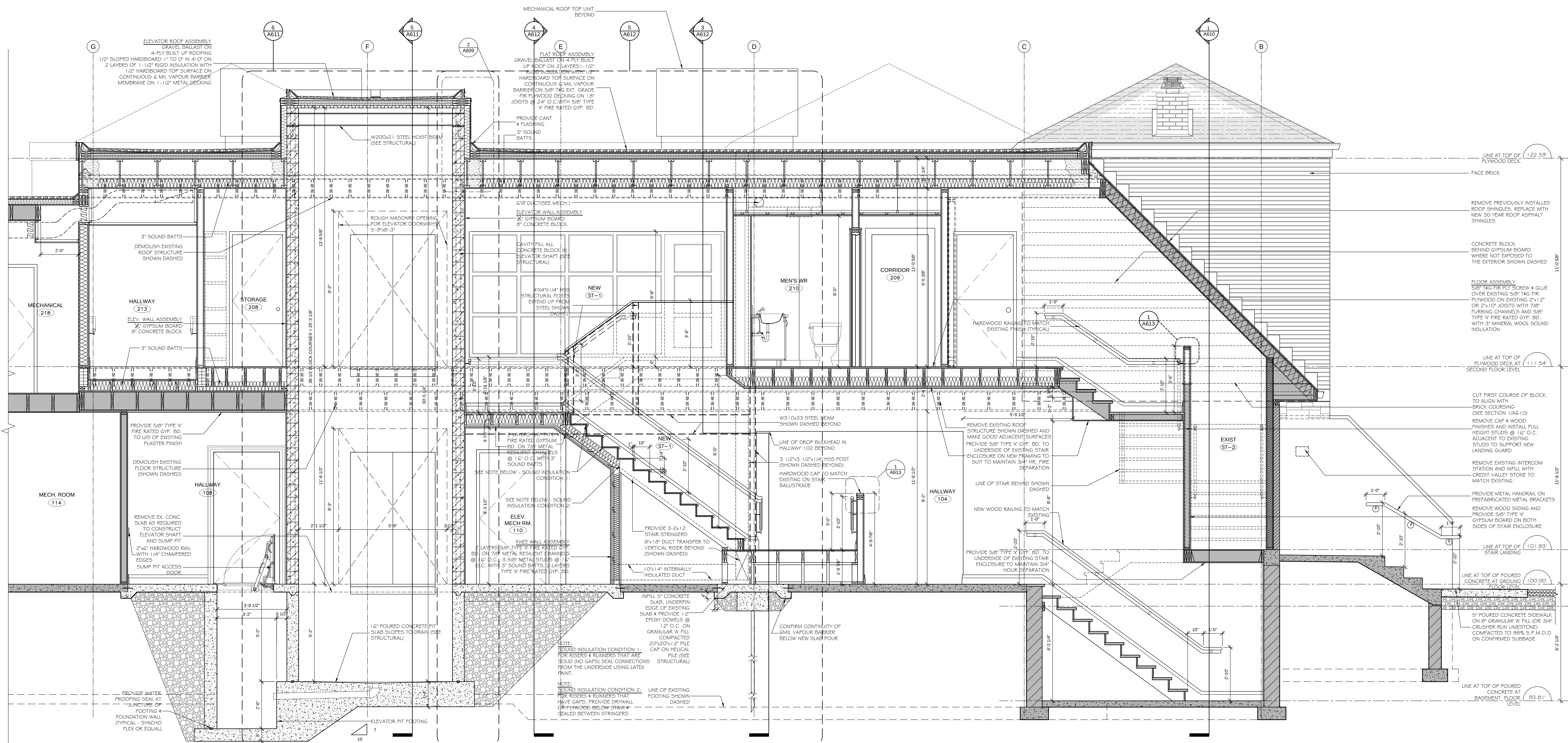
1 SECTION No. 17 A609 1/2" = 1'-0"
