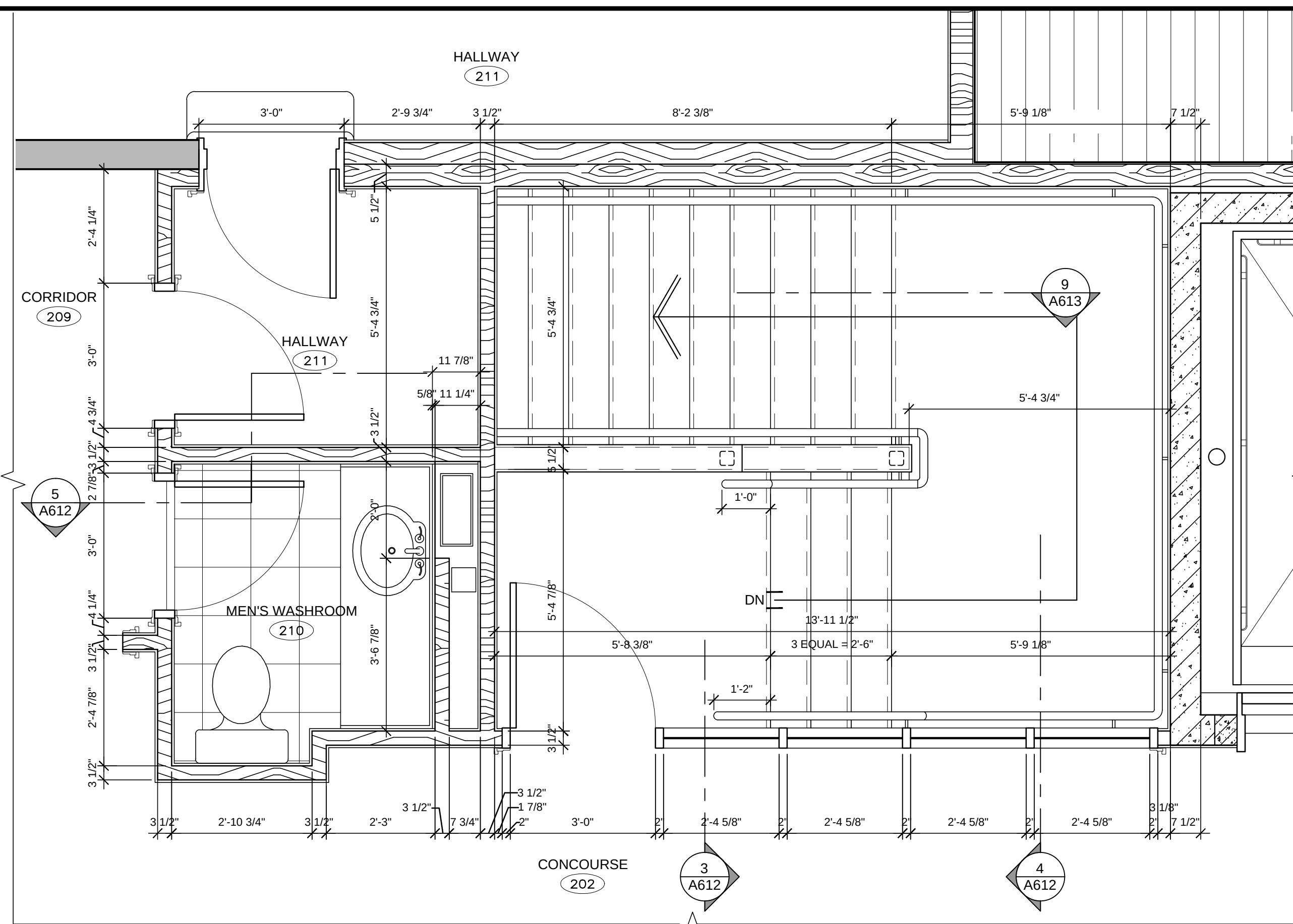
2 ST-1 UPPER PLAN A612 1/2" = 1'-0"
