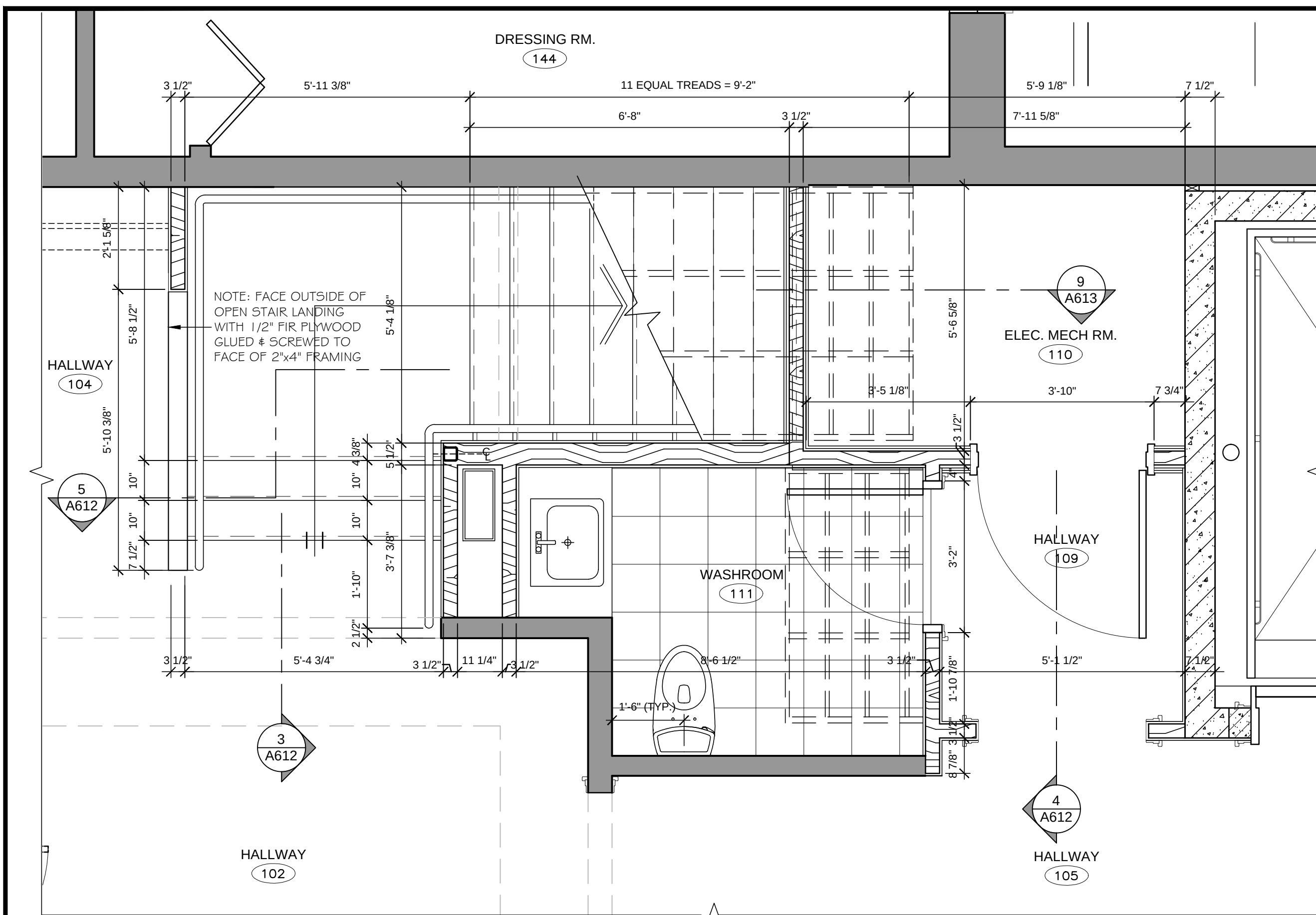
1 ST-1 LOWER PLAN A612 1/2" = 1'-0"
