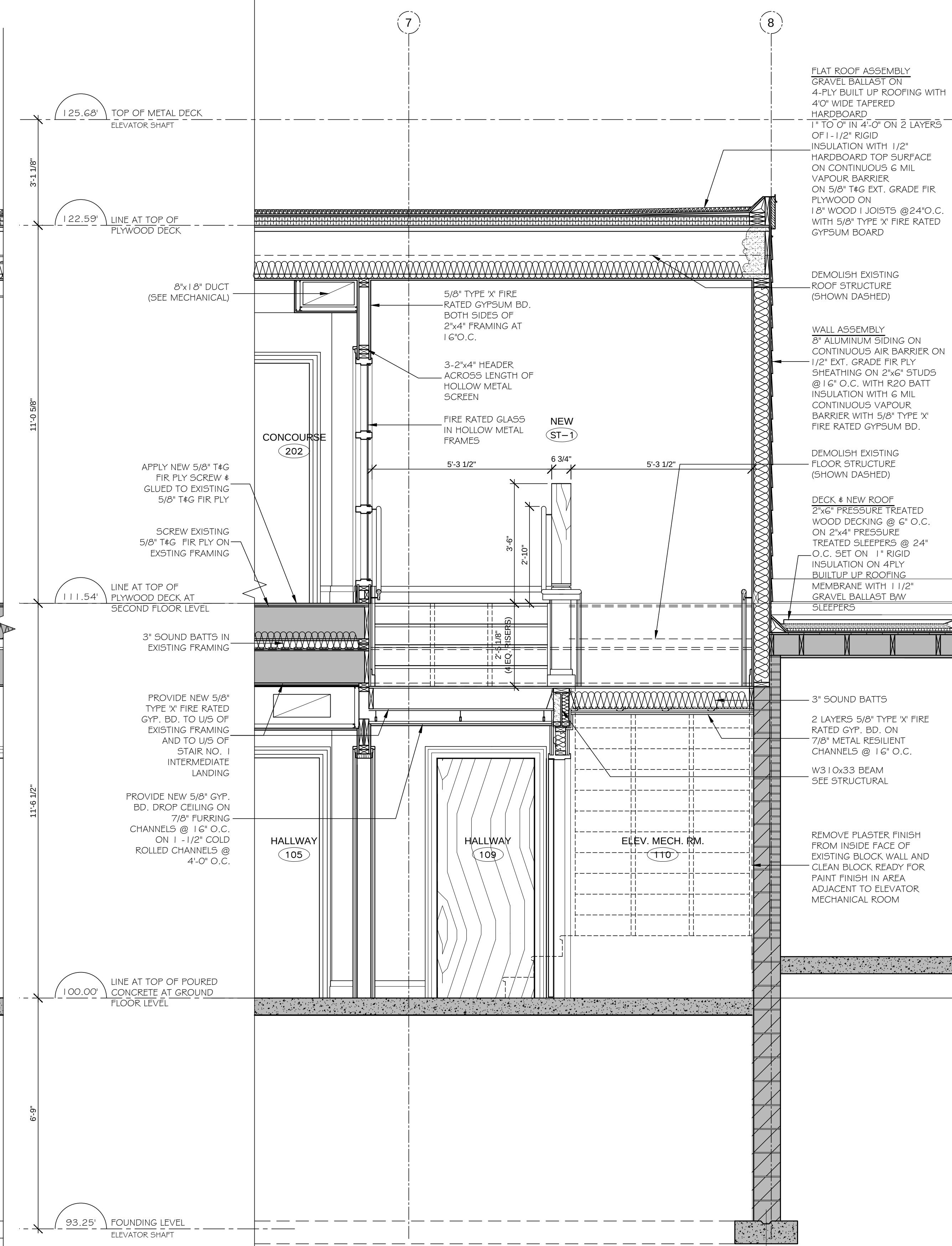
4 ST-1 SECTION A612 1/2" = 1'-0"
