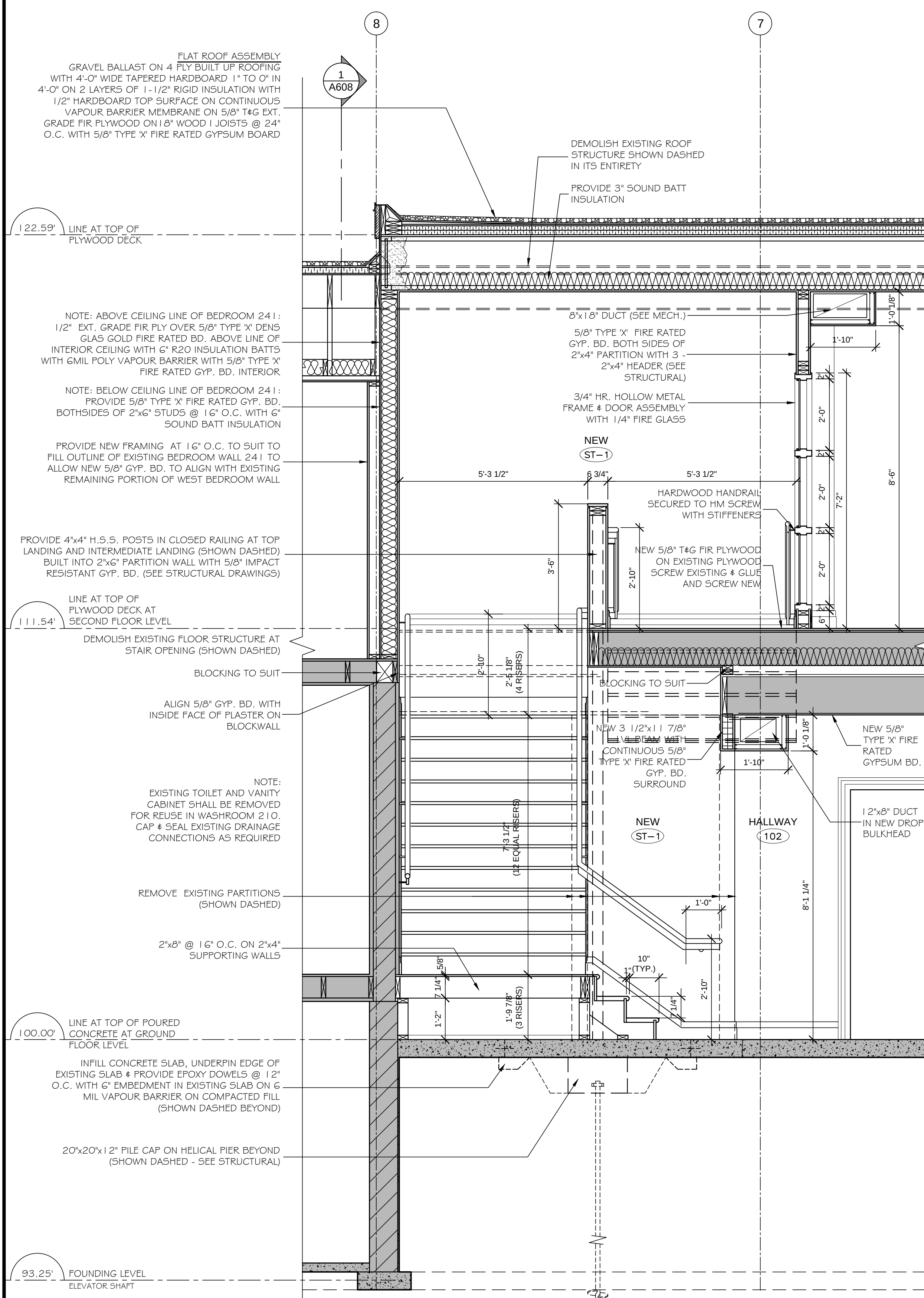
3 ST-1 SECTION A612 1/2" = 1'-0"
