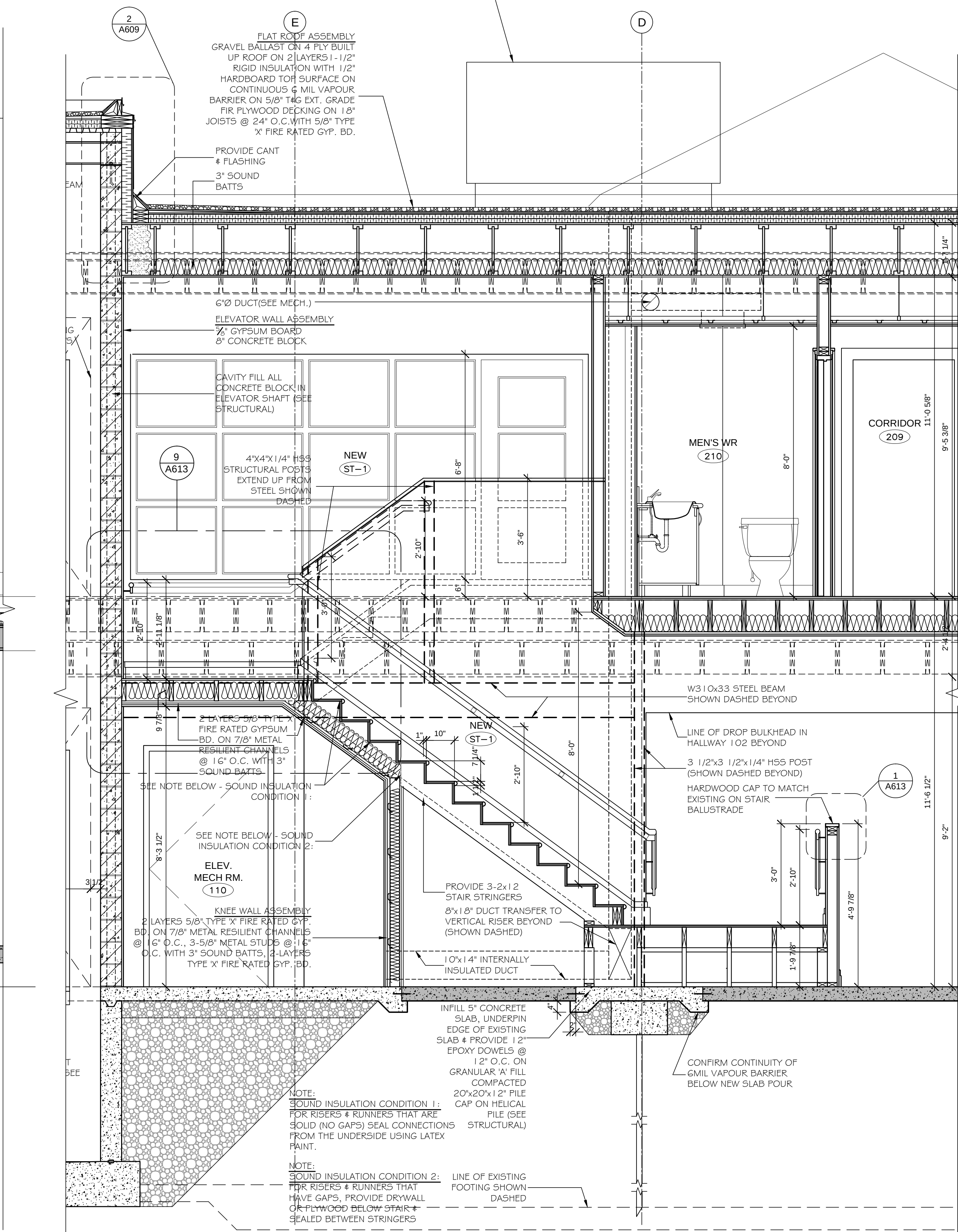
5 ST-1 SECTION A612 1/2" = 1'-0"
