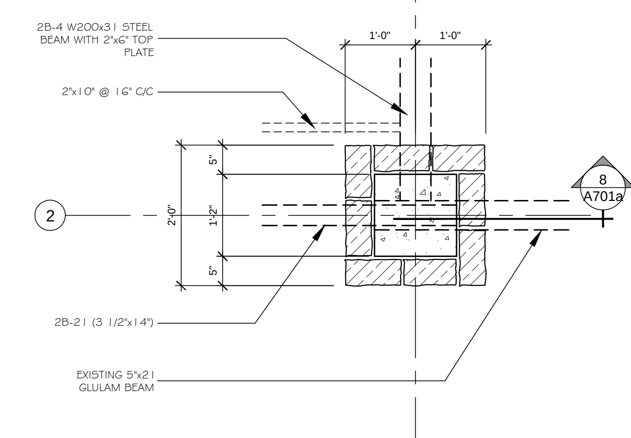
PIER J2 - UPPER PLAN
