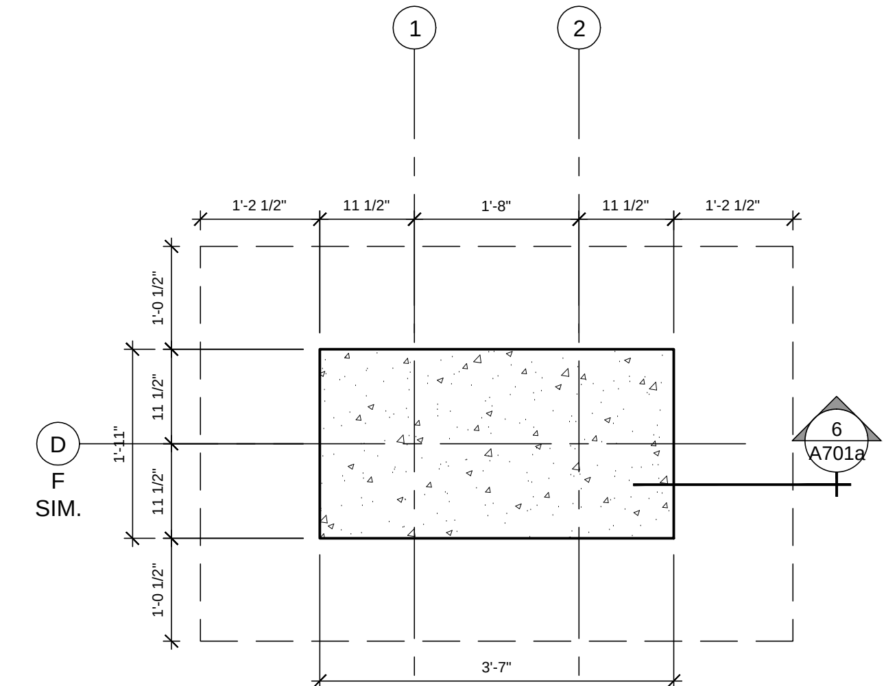
PIER D1.2, PIER F1.2 (SIM) - FOUNDATION PLAN
