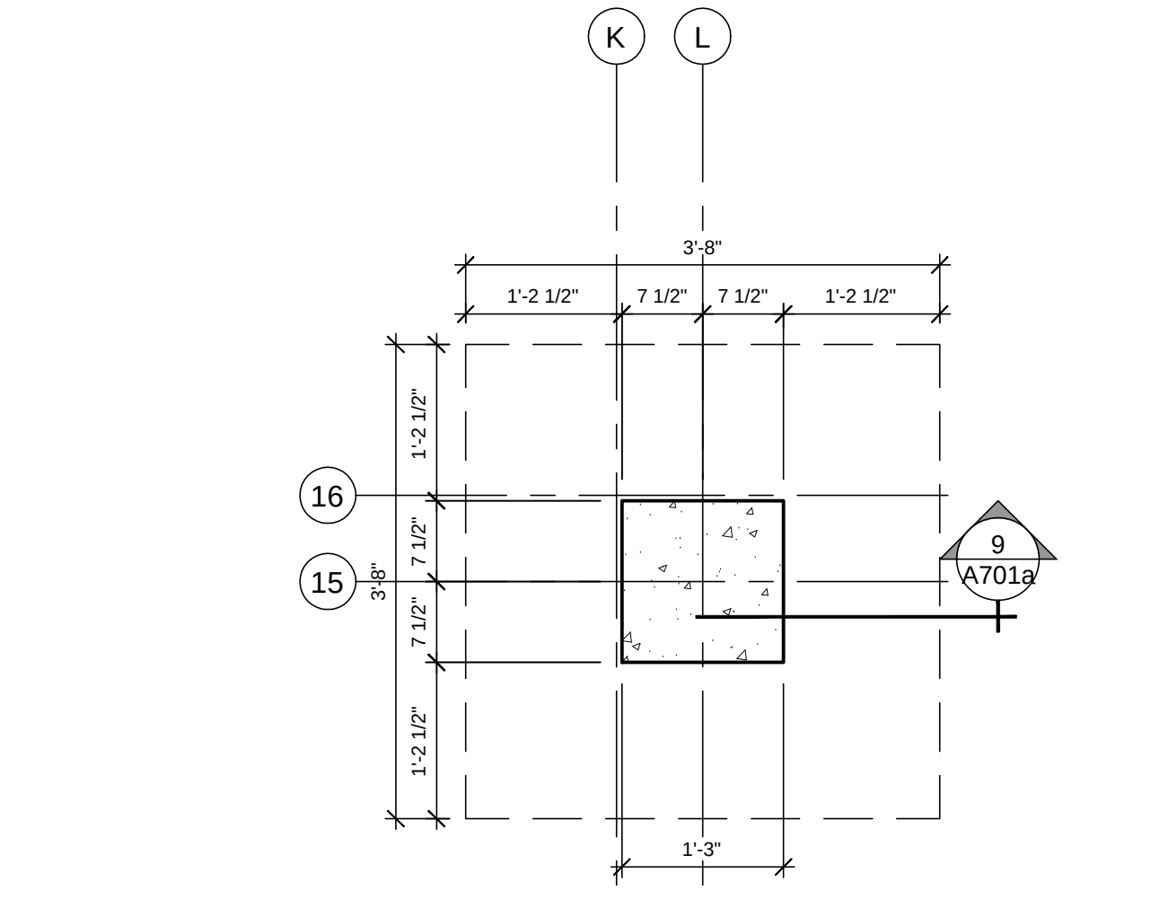
PIER L15 - FOUNDATION PLAN
