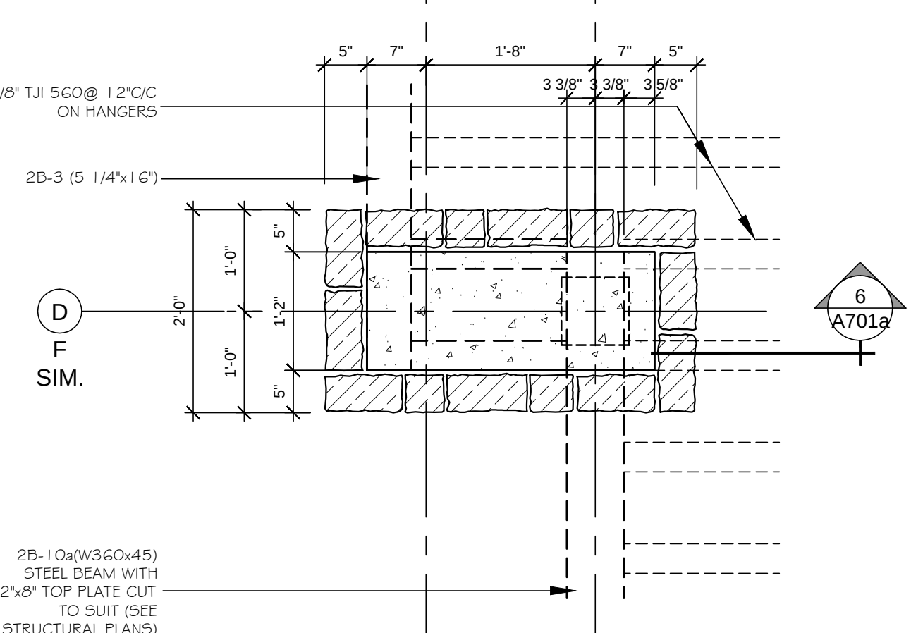
PIER D1.2, PIER F1.2 (SIM) - UPPER PLAN
