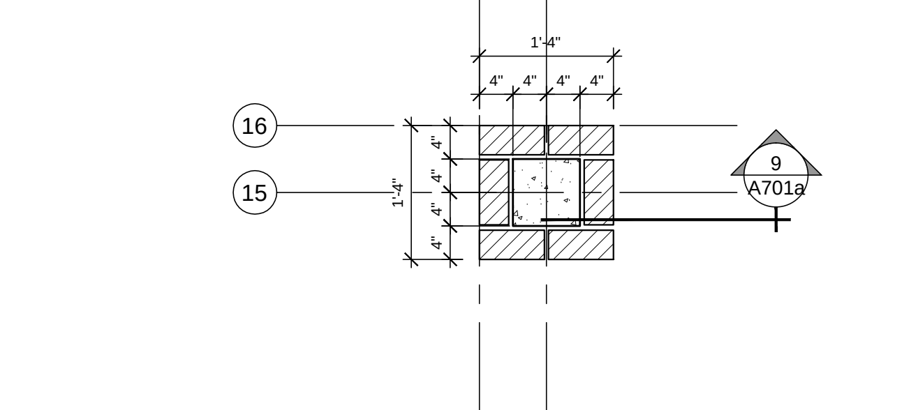
PIER L15 - FOUNDATION PLAN
