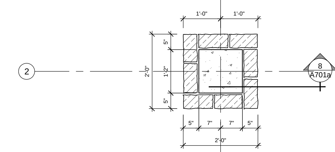
PIER J2 - FOUNDATION PLAN
