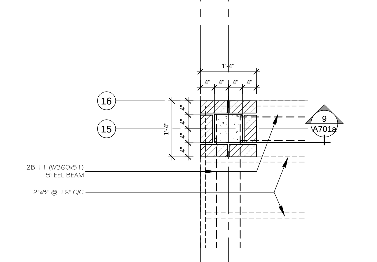
PIER L15 - UPPER PLAN
