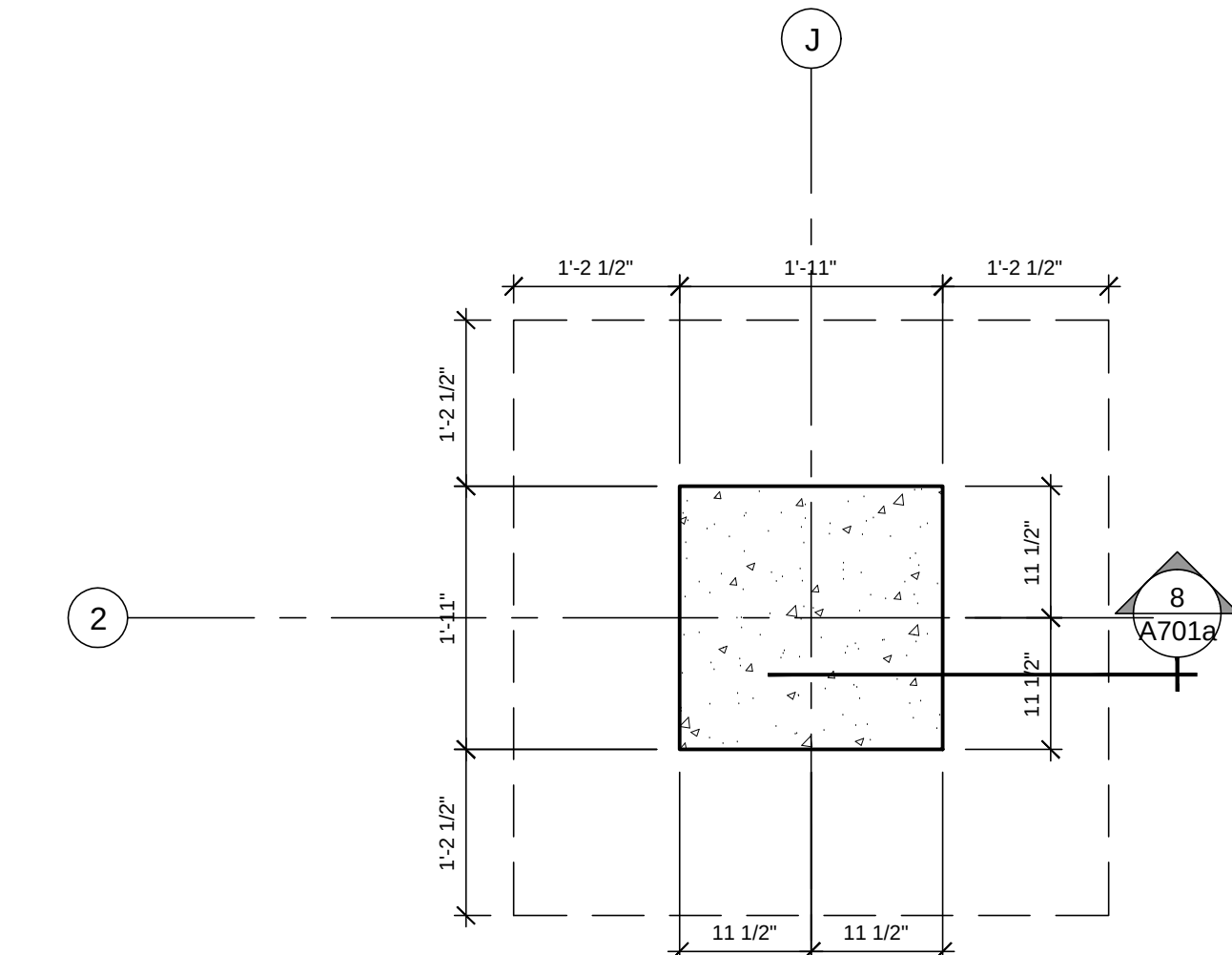
PIER J2 - FOUNDATION PLAN
