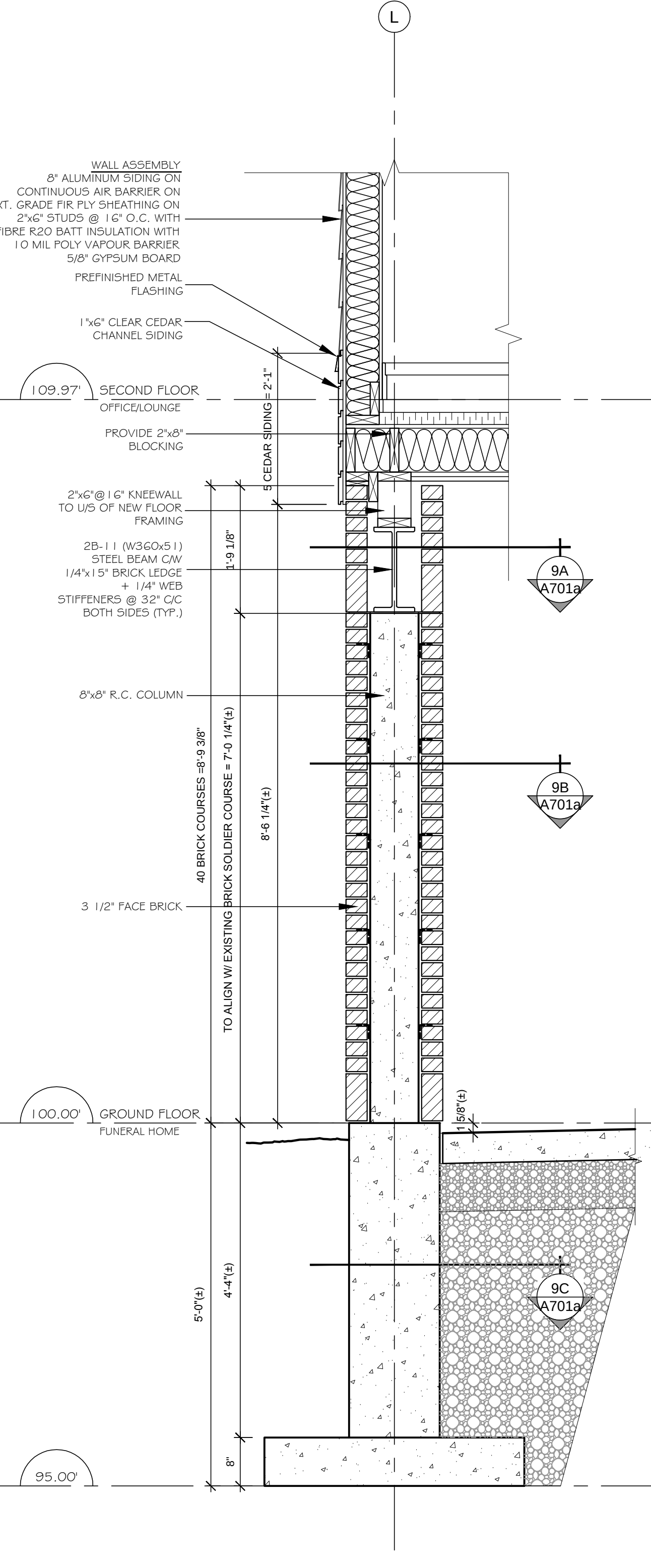
PIER L15 - SECTION
