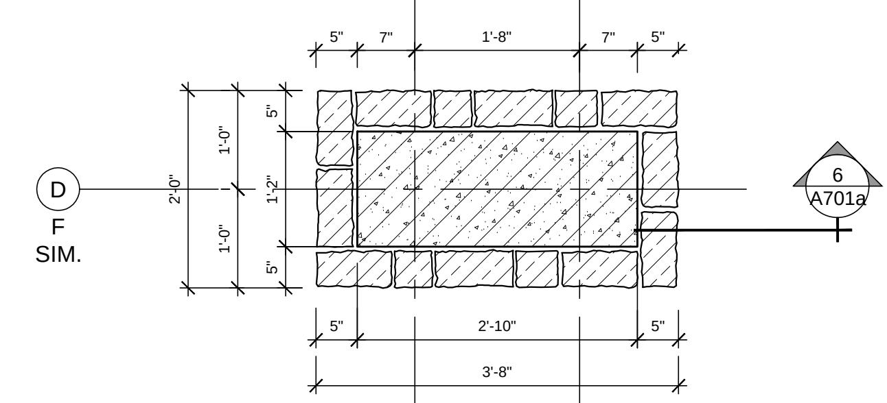
PIER D1.2, PIER F1.2 (SIM) - FOUNDATION PLAN
