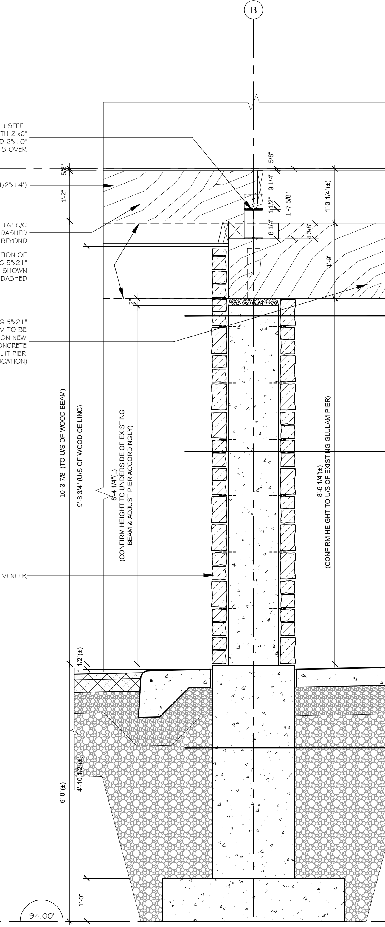
PIER J2 - SECTION
