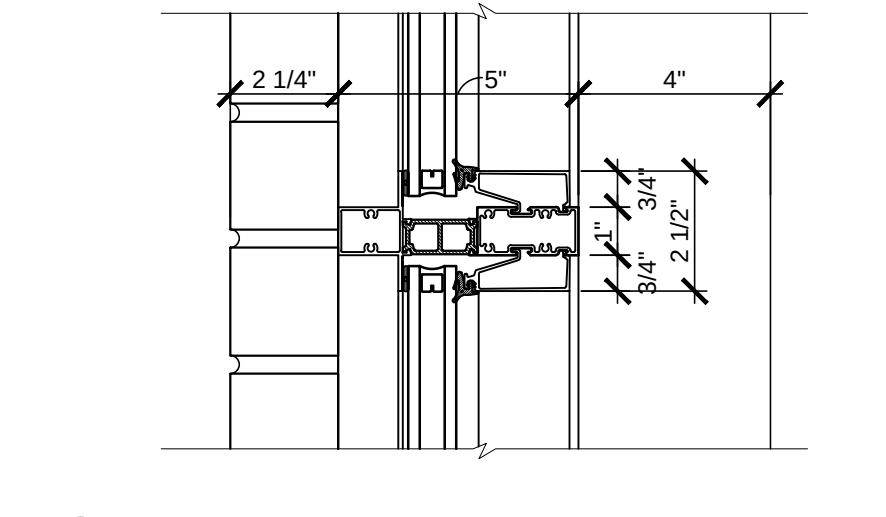
WINDOW MULLION (TYP) SCALE: 3"=1'-0"
