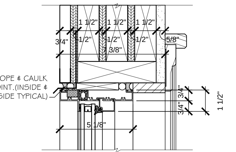
WINDOW HEAD (TYP) SCALE: 3"=1'-0"
