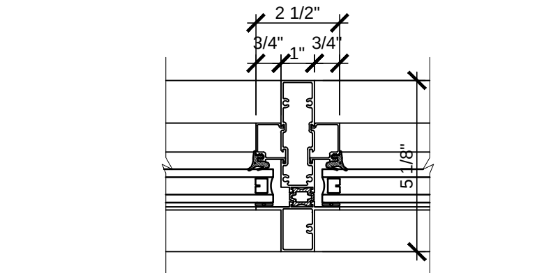
WINDOW MULLION (TYP) SCALE: 3"=1'-0"
