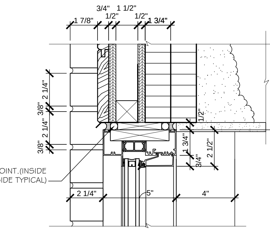
WINDOW HEAD (TYP) SCALE: 3"=1'-0"
