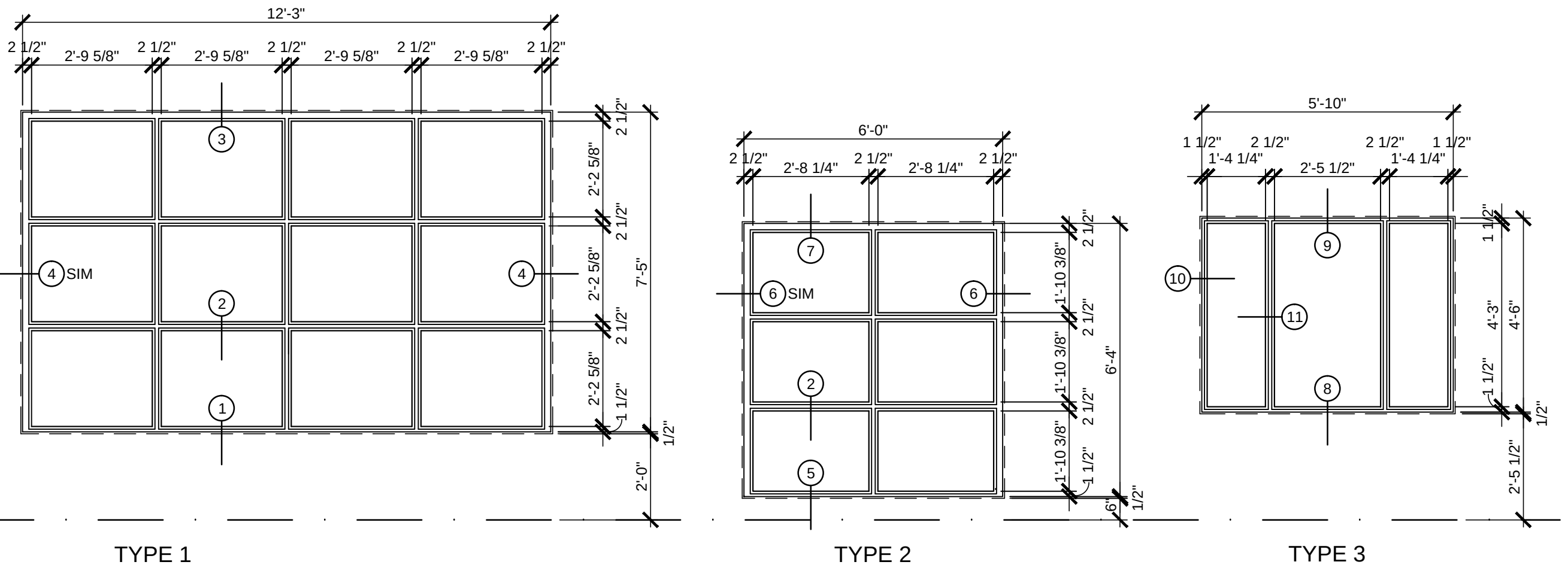
WINDOW ELEVATIONS SCALE: 3/8"=1'-0"
